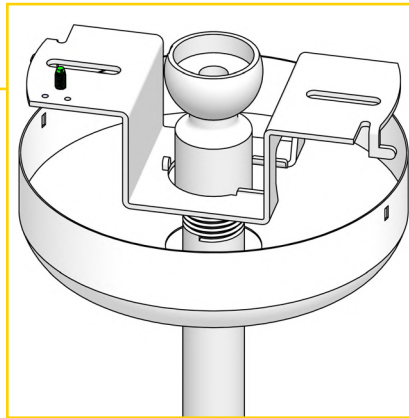
Pendant Mount Includes Canopy Swivel Kit
